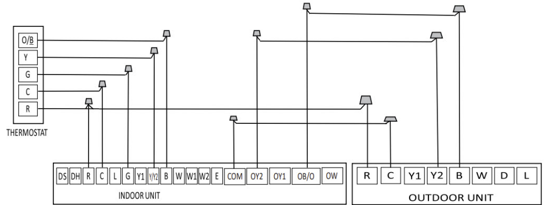
Wiring for 1H & 1C Thermostat
