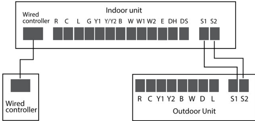
Connection Method A: Full Communication
