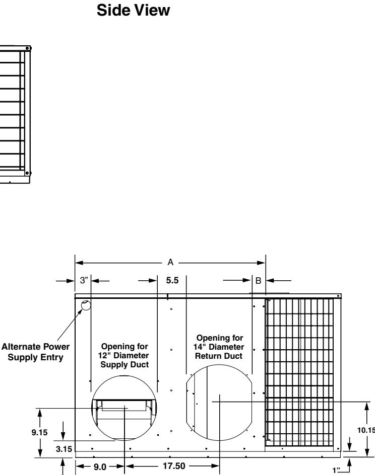
Back (Duct) View (3.5-5 Ton)
